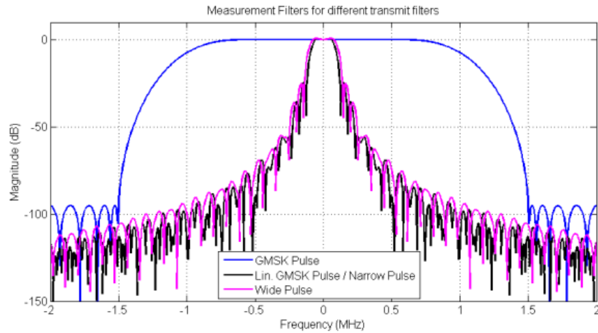
Fig. 2-27: Magnitude Responses of Measurement Filters for Demodulation Measurements
