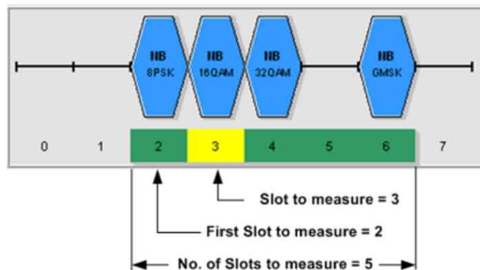
Fig. 2-22: Concept of "First Slot to measure", "Number of Slots to measure" and "Slot to Measure"
