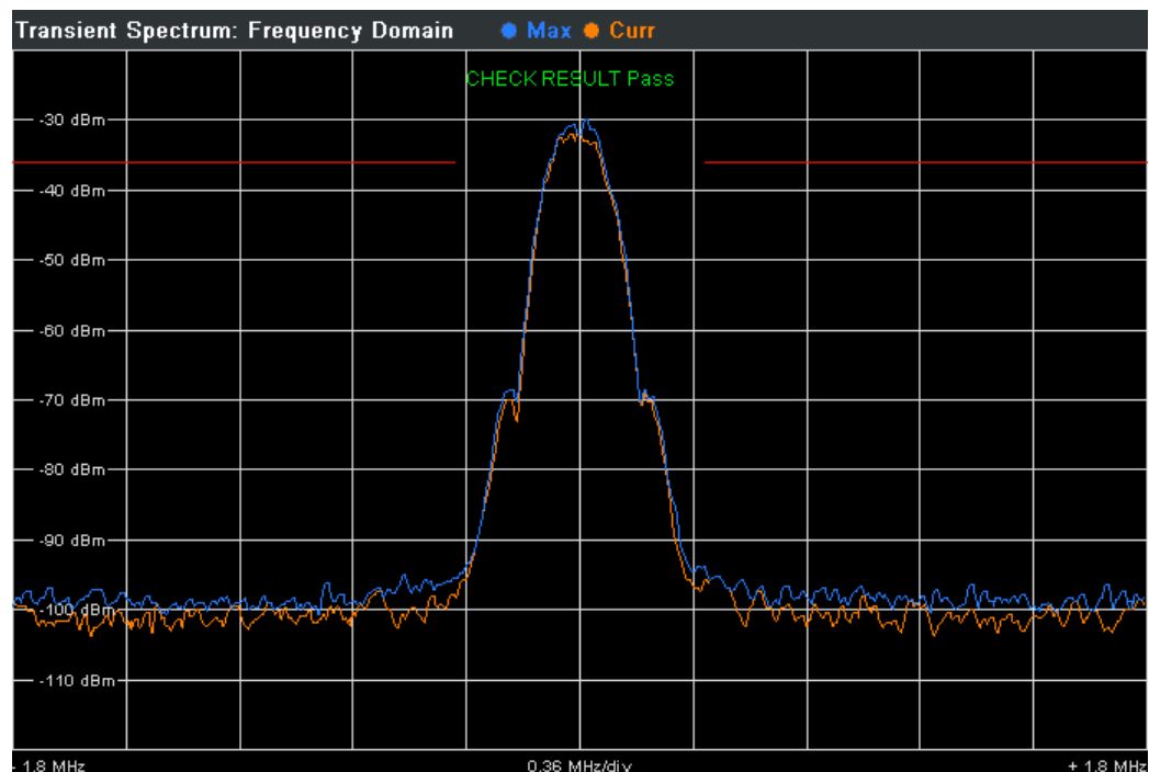
Fig. 2-14: Frequency Domain of Transient Spectrum with traces and limits (red)
