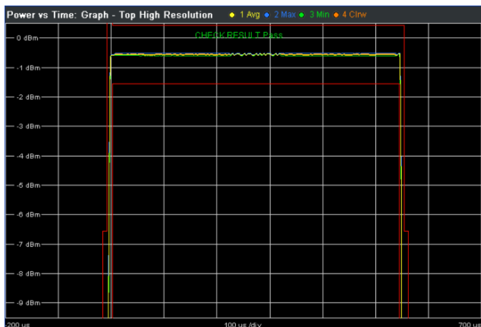
Fig. 2-10: Top High Resolution view in Power vs Time
