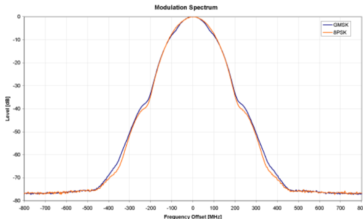
Fig. 2-19: GMSK and 8PSK modulation spectrum
