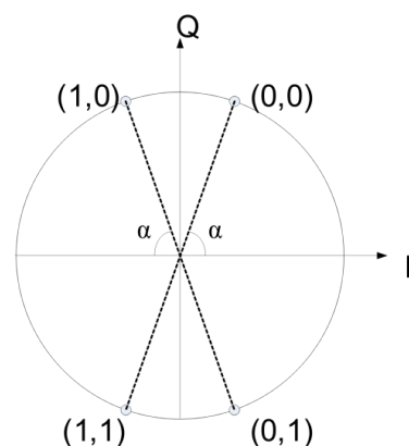
Fig. 2-21: AQPSK constellation [reproduced from 3GPP change request document GP-100275].
