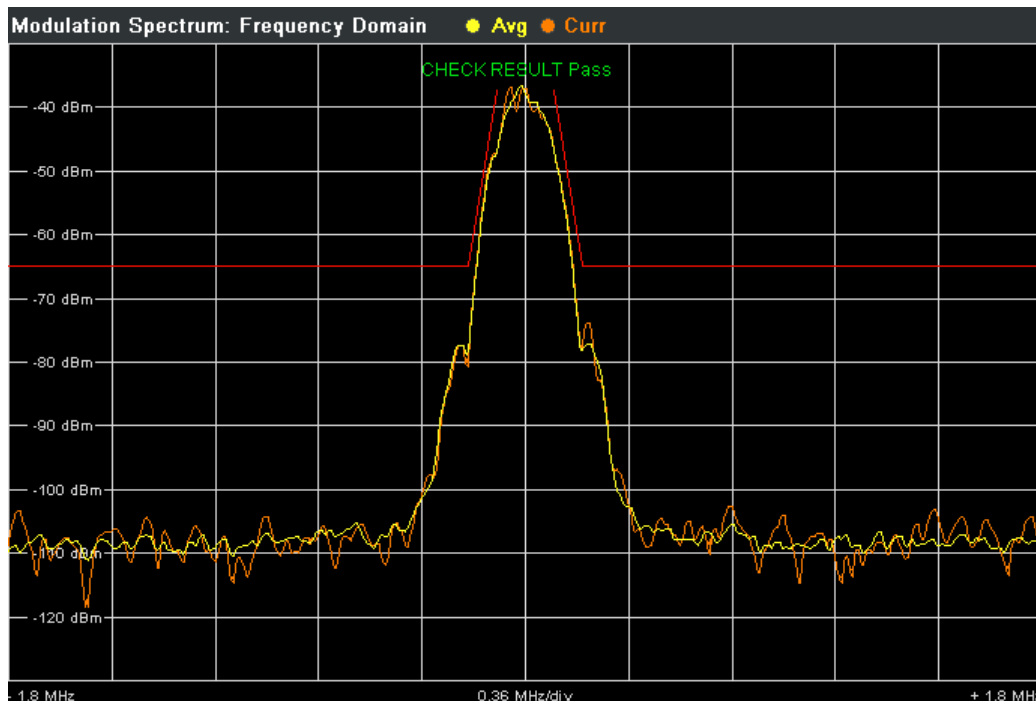
Fig. 2-12: Frequency Domain of modulation spectrum with traces and limits (red)
