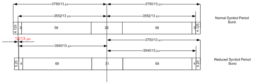
Fig. 2-31: Timing alignment between normal symbol period and reduced symbol period bursts
