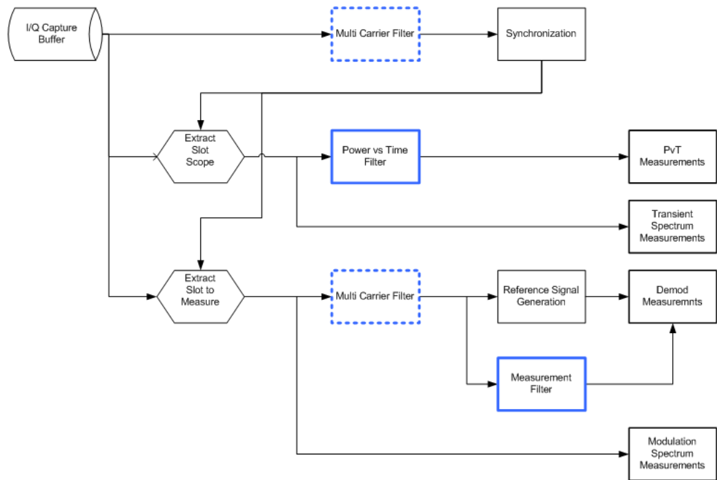
Fig. 2-23: Signal flow diagram highlighting filtering operations
