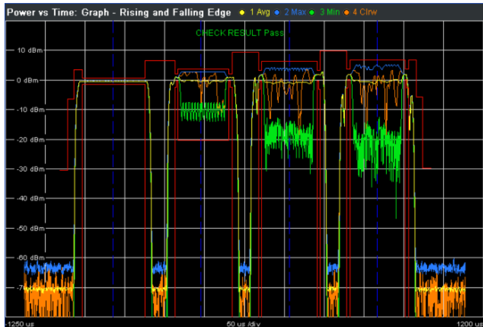
Fig. 2-9: Rising and Falling Edge view in Power vs Time
