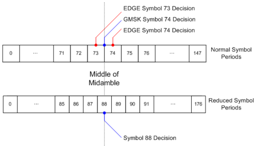
Fig. 2-32: Middle of midamble for normal and reduced symbol period bursts.
