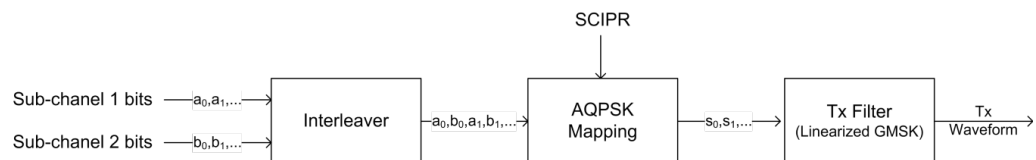
Fig. 2-20: AQPSK modulation scheme for GSM systems
