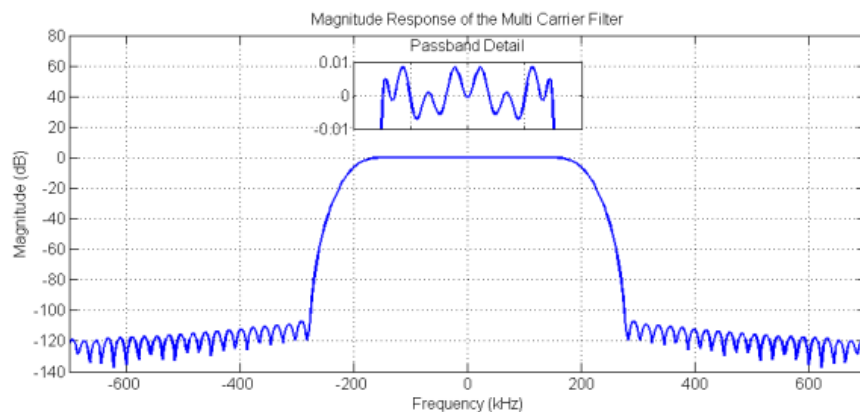
Fig. 2-24: Frequency Response of the Multi Carrier Filter
